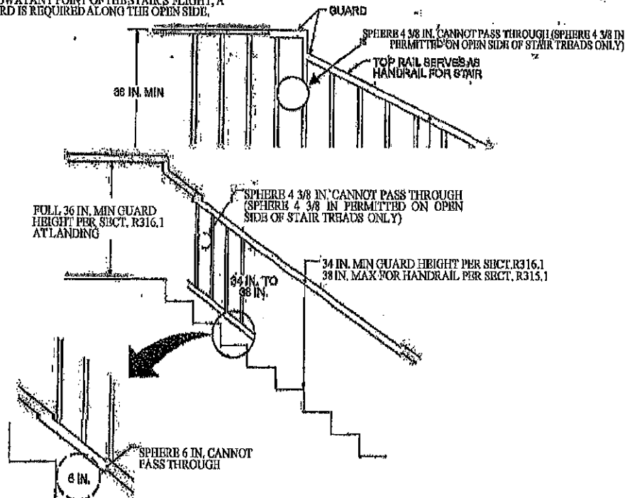
Figure R312 GUARD REQUIREMENTS
